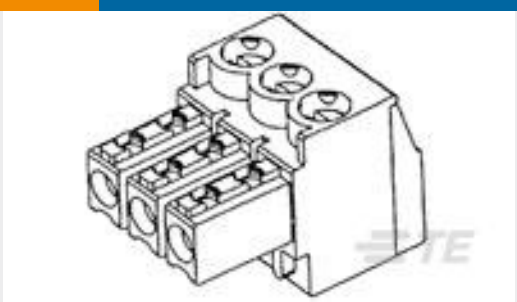
TE Part #1-284506-2 12 POS TERMI-BLOK PLUG STAC 3,
