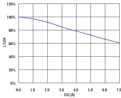
HE06184R7MS□
