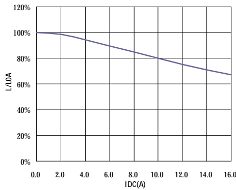
HE06181R0MS□
